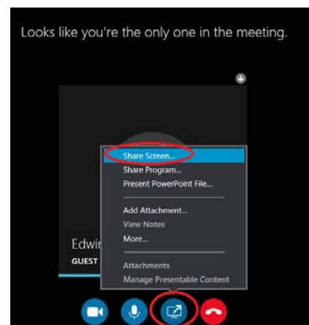
Figure 9 Sharing Content
